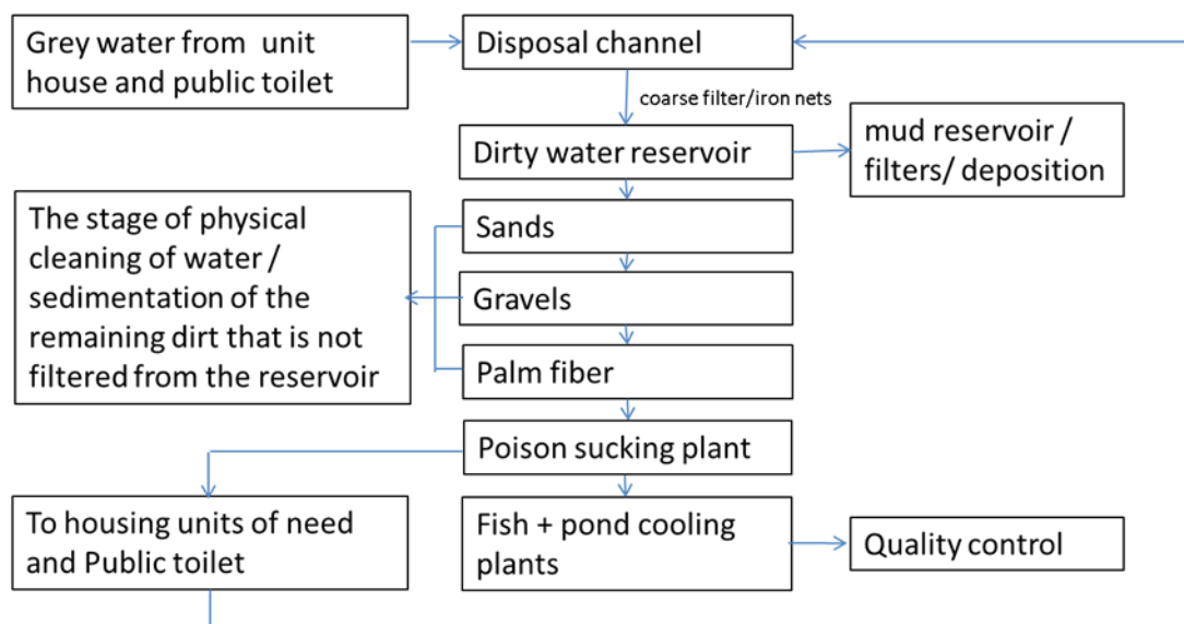
Figure 13. Scheme of grey water treatment horizontal flow
